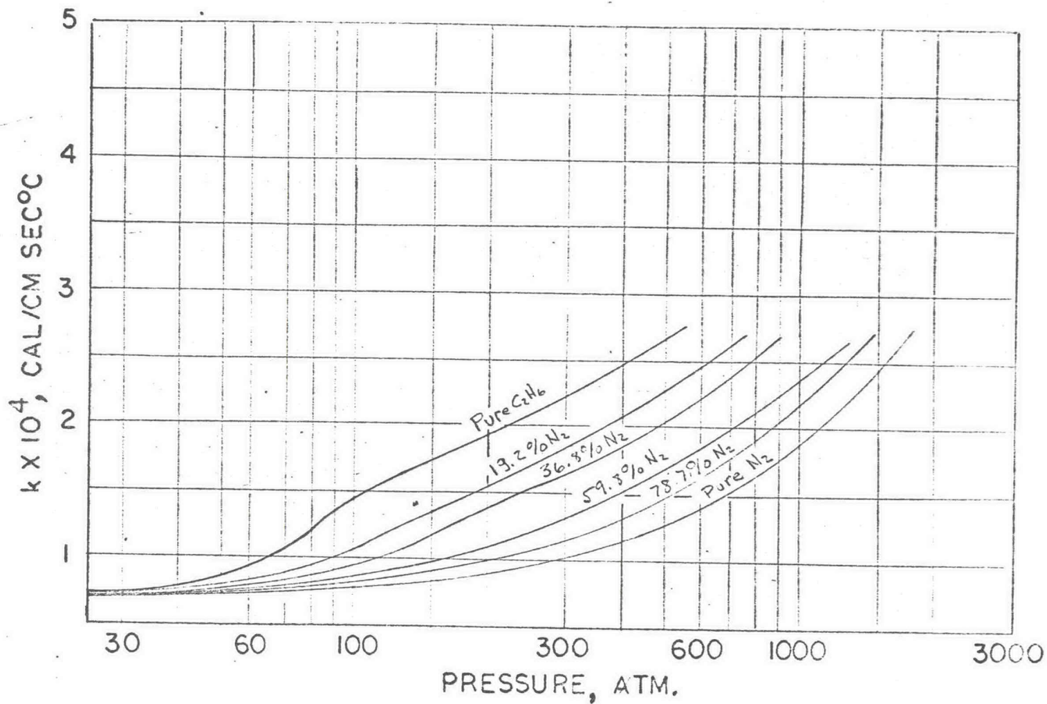
FIGURE 8. THERMAL CONDUCTIVITY OF N 2 -C 2 H 6 MIXTURES AT 75°C
